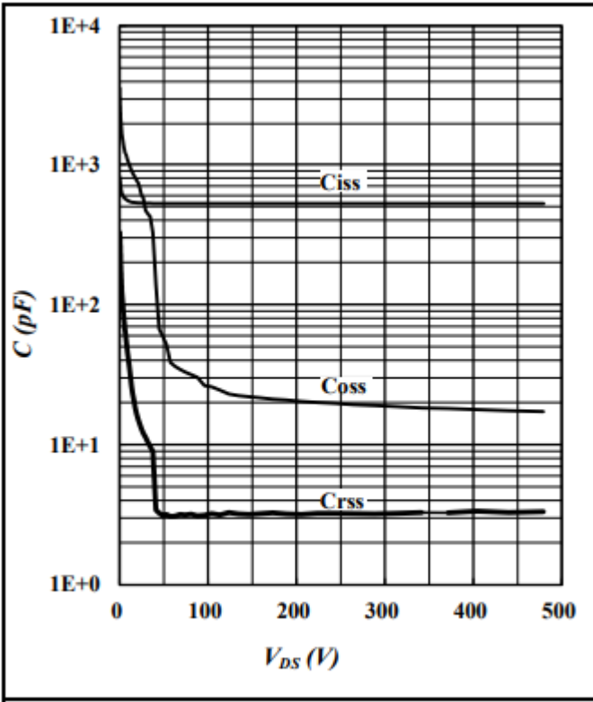
Fig.5 Typ. Capacitance vs. V_{DS}
