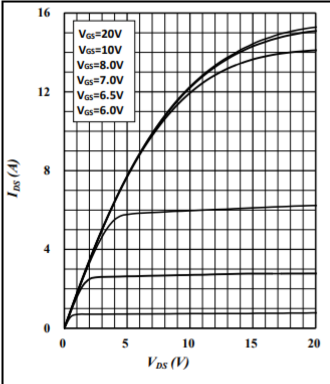
Fig.1 Typ. Output Characteristics T_j = 25\text{ }^\circ\text{C}
