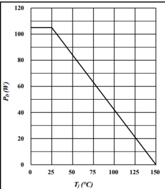
Fig.7 Power Dissipation Derating Curve
