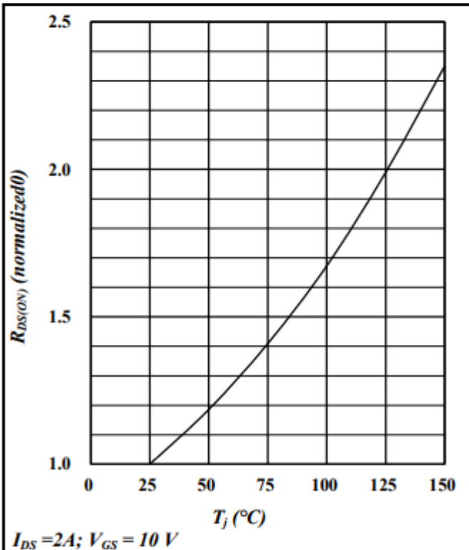
Fig.3 R_{DS(ON)} vs. Junction Temperature
