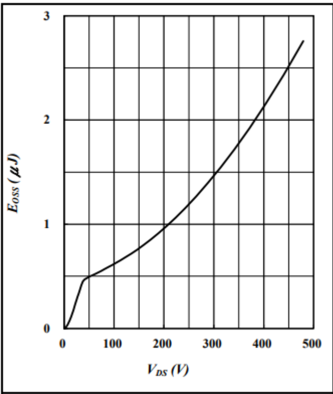
Fig.11 Eoss Curve
