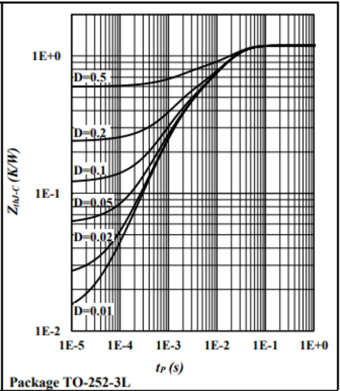
Fig.10 Z_{thJ-C} , D = tP / T
