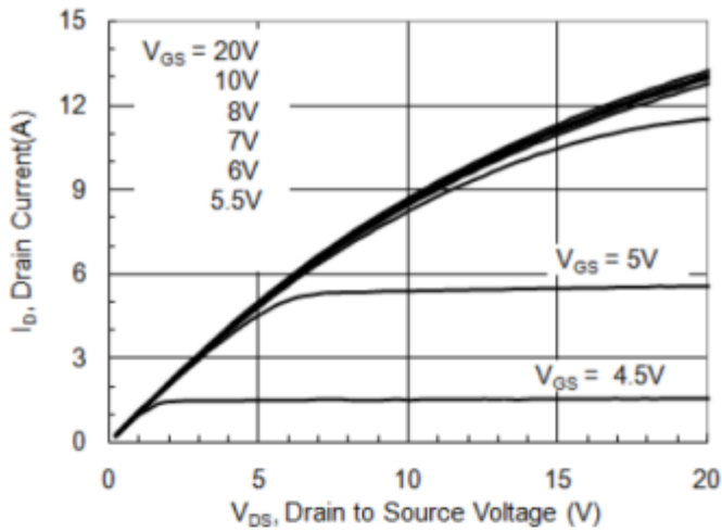
Fig1. Output characteristics
