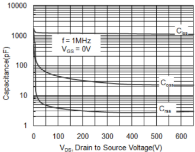
Fig 4. Capacitance Characteristics
