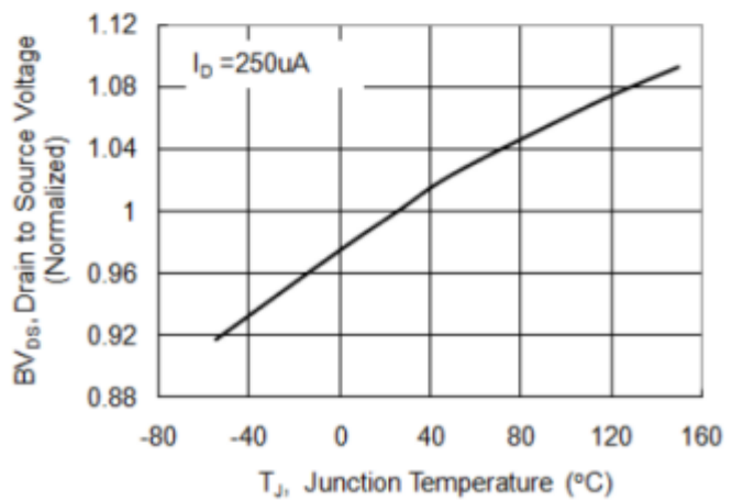
Fig 6. BV_{DSS} vs junction temperature
